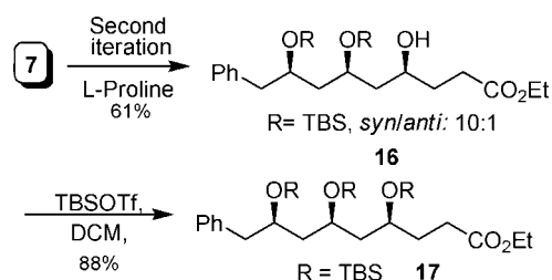
Scheme 4. Second Iteration for Synthesis of Triol a
