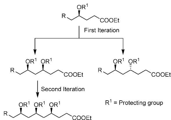
Figure 1. Iterative strategy for polyol synthesis.
