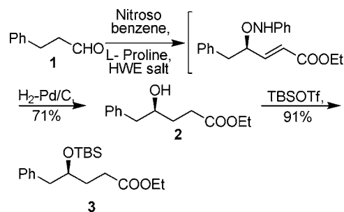
Scheme 1. Synthesis of \gamma -Hydroxy Ester
