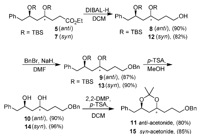
Scheme 3. Relative Stereochemistry Determination
