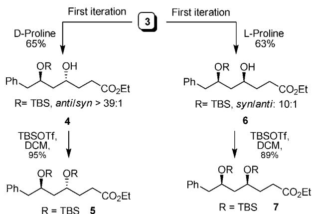
Scheme 2. First Iteration for Synthesis of Diol a
